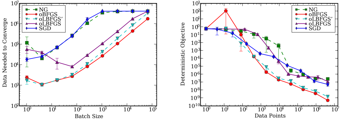
Figure 2: Average performance (with standard errors) of stochastic gradient methods on the non-realizable quadratic (16) with \sigma = 10^{-2} over 10 matched random replications. Left: number of data points needed to converge to f(\theta) < 10^{-5} , up to a limit of 2^{22} , vs. batch size b . Right: deterministic loss f(\theta) vs. number of data points seen, at the optimal batch size for each algorithm. All methods used (7) with \eta_0 and \tau tuned for fastest convergence at small batch sizes: \eta_0 = b/(b+2), \tau = 10^4 (SGD); \eta_0 = 0.04, \tau = 20 (NG); \eta_0 = b/(b+2), \tau = 20 (oBFGS); \eta_0 = 0.1 \cdot b/(b+2), \tau = 2 \cdot 10^4 (oLBFGS); \eta_0 = b/(b+2), \tau = 10 (oLBFGS'); \lambda, c, m as in Figure 1.
