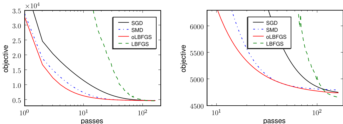
Figure 3: Left: loss on vs. number of passes through the CoNLL-2000 training set, for 4 gradient methods. Right: enlargement of final portion of the curves. Parameter values: SGD: \eta = 0.1 ; SMD: \boldsymbol{\eta}_0 = 0.1, \mu = 0.1, \lambda = 1 ; LBFGS: m = 5 ; oLBFGS: m = 5 , (7) with \tau = 10^4, \eta_0 = \lambda = 1 .
