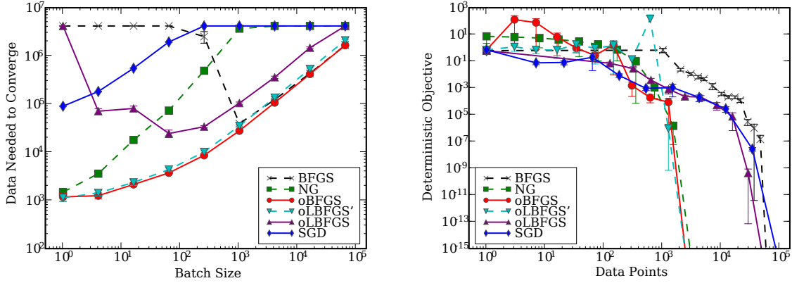
Figure 1: Average performance (with standard errors) of stochastic gradient methods on our model problem over 10 matched random replications. Left: number of data points needed to reach f(\theta) \leq 10^{-15} , up to a limit of 2^{22} , vs. batch size b . Right: deterministic loss f(\theta) vs. number of data points seen, at the optimal batch size for each algorithm. All methods used \eta_t = b/(b+2) (tuned for best performance of SGD) except NG, which required (7) with \eta_0 = 1 and \tau = 100 . BFGS parameters: \lambda = 0, c = 0.1; m = 4 (oLBFGS) resp. 10 (oLBFGS').
